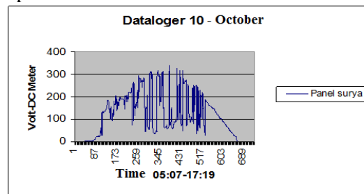
Figure 4.1 Plot of sun intensity data from sunrise–sunset obtained on October-10.
