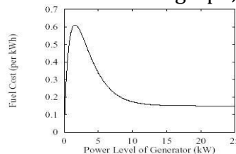
Figure 5.1 Graph of the relationship between generator power levels and fuel prices.
