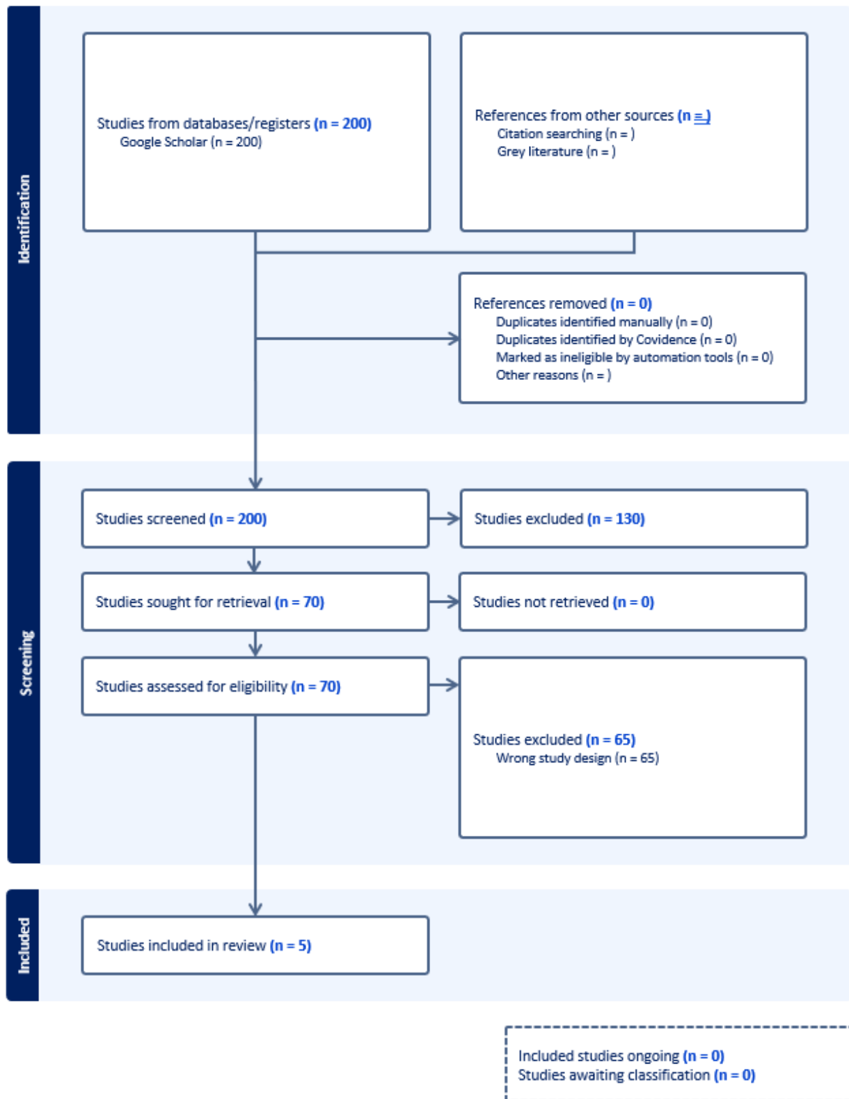
Gambar 3 Prisma Convindence
